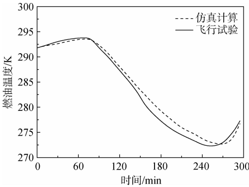
图 7 外翼内隔舱燃油温度计算结果与试验数据对比 Fig. 7 Comparison between calculated results of fuel temperature in inner compartment tank of outer wing and experimental data
