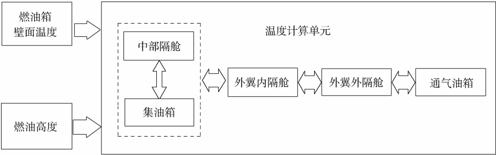
图 3 基于 Simulink 的油箱建模流程 Fig. 3 Fuel tank modeling process based on Simulink
