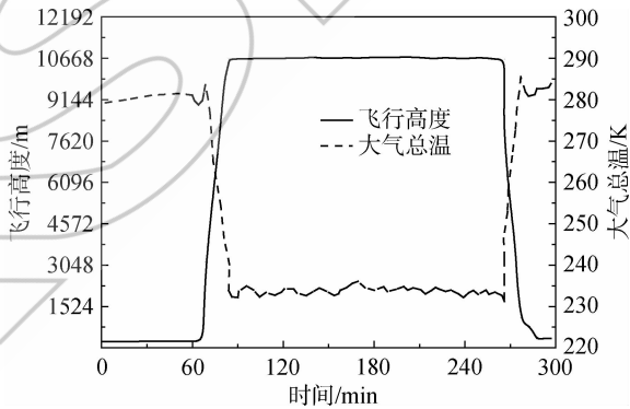
图 6 飞行高度和大气总温的变化规律(标准天长航程) Fig. 6 Change rule of flight altitude and total atmospheric temperature (long range, international standard atmosphere)
